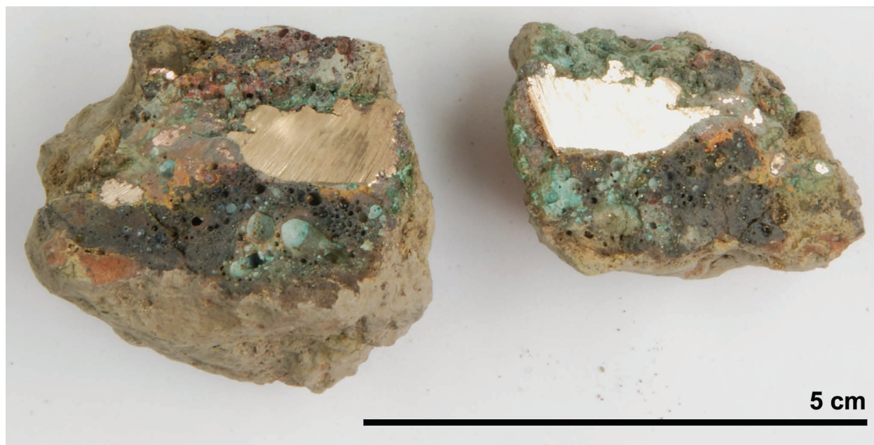
Figure 5: Section of hearth fragment Fd. Nr. 1032. The section reveals bronze casting waste and copper prills and frothy vitrified ceramic and glassy slag.
