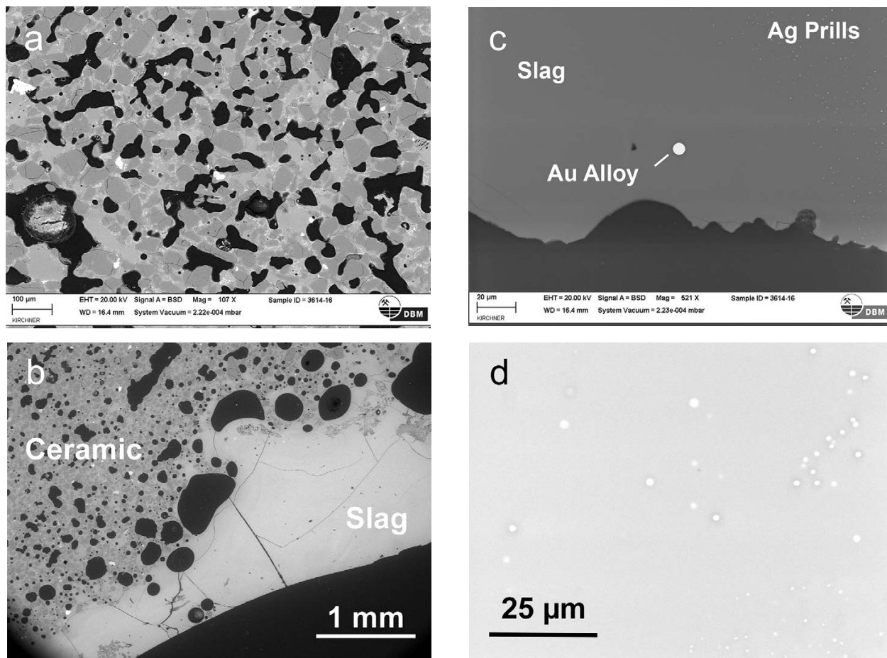
Figure 2: Crucible Fd. Nr. 410 SEM-backscatter images. a) Crucible ceramic microstructure. Silt to fine sand-sized quartz, feldspars and micas held together by a network of glass. b) Vitreous slag and crucible ceramic. c) Gold alloy prill in glassy slag and region with µm to sub-µm-sized silver prills. d) Silver prills in slag.
