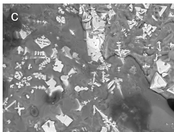
Figure 4: Crucible Fd. Nr. 3342 SEM-backscatter images. a) Section showing the frothy vitrified repair layer and the denser crucible ceramic. The white areas are silver corrosion products and metallic silver in the crucible ceramic pores. b) Mounted and polished section showing the repair layer and the crucible ceramic. c) Magnetite crystals in the glass on the crucible exterior. No scale.
