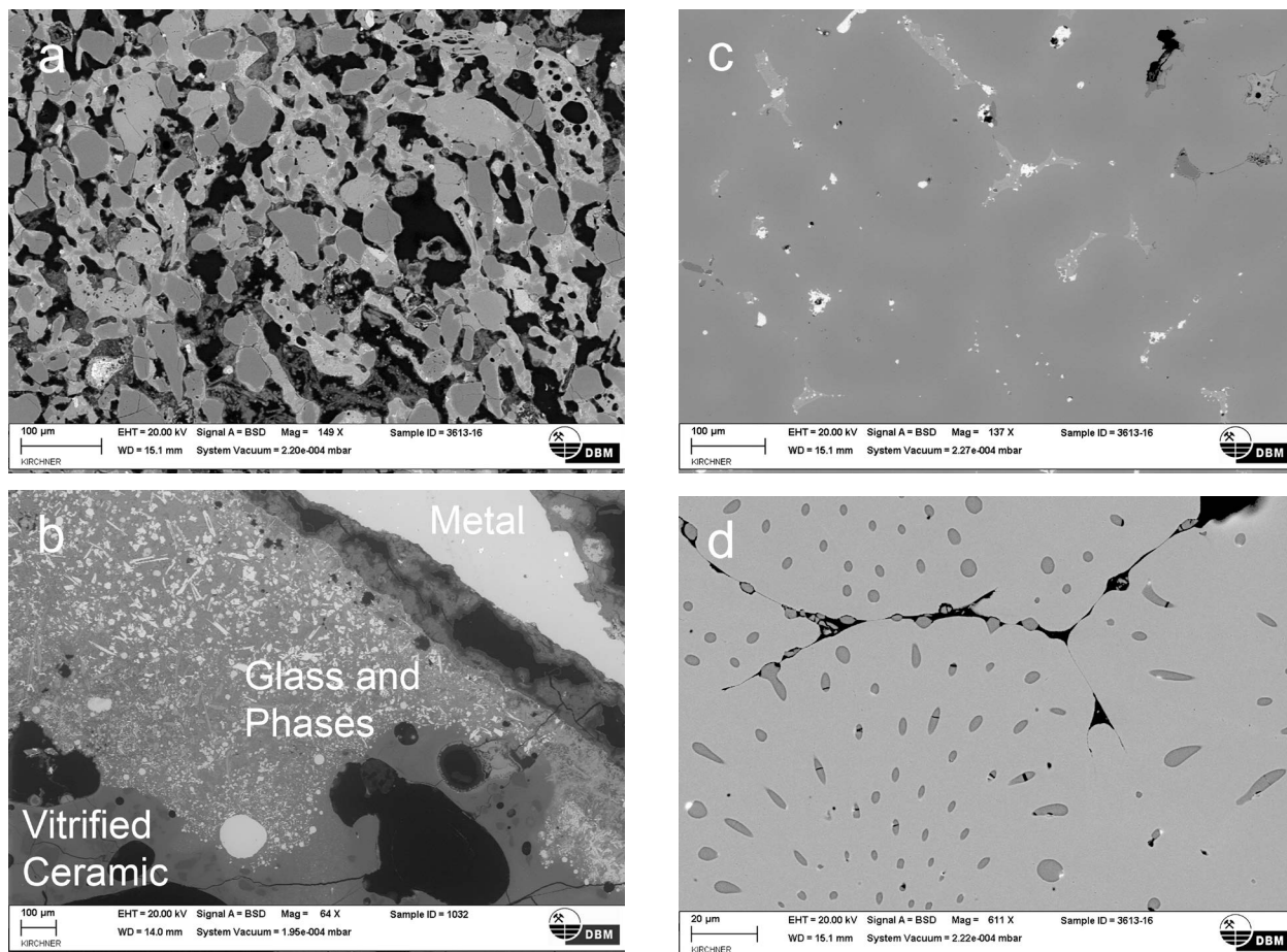
Figure 6: Hearth fragment Fd. Nr. 1032 SEM-backscatter images. a) Microstructure of the technical ceramic with abundant silt to fine sand-sized quartz, feldspars and micas held together by a network of glass. b) Glassy layer between ceramic and bronze metal. The tin oxide phases in the glassy layer show that there was a high temperature interaction with the bronze. c) Microstructure of bronze spill. Lead (white) is found at the grain boundaries along with regions of high tin (alpha+delta). d) Prill of copper with copper eutectic showing that the copper was in a liquid state.
